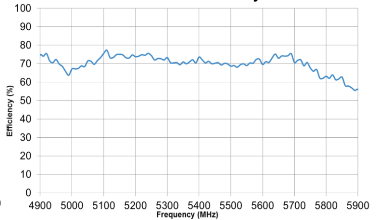
5 GHz Efficiency
