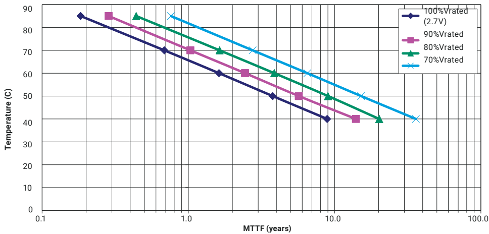
Expected Lifetime at Various Voltages SCC Series, 2.7V Rated
