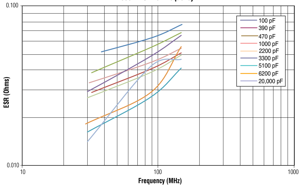
800 H ESR vs. Frequency
