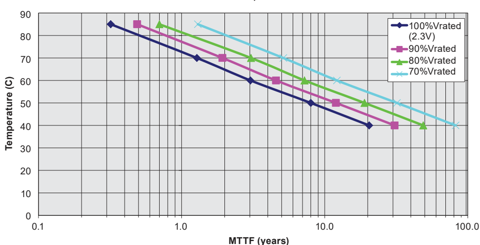
Expected Lifetime at Various Voltages SCC Series, 2.3V Rated
